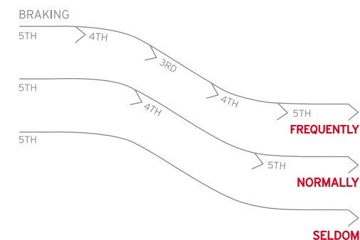
ADAPTIVE SHIFT CONTROL GOING DOWNHILL
